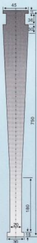
模柄 I Punch support I
